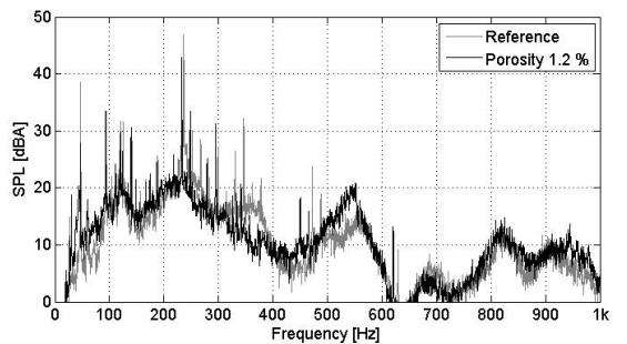
Fig. 7 Comparison of noise spectra of the machine room with and without the PPS of porosity 1.2 %
