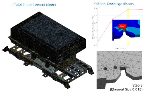
Fig. 2 Whole model and mesh determination method
