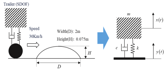
Fig. 6 Equivalent bump shock environmental modeling
