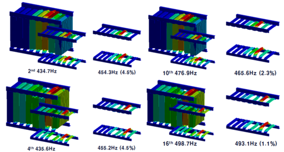
Fig. 10 Mode shape(specific model/analysis model)
