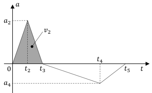
Fig. 3 BV043 triangle wave
