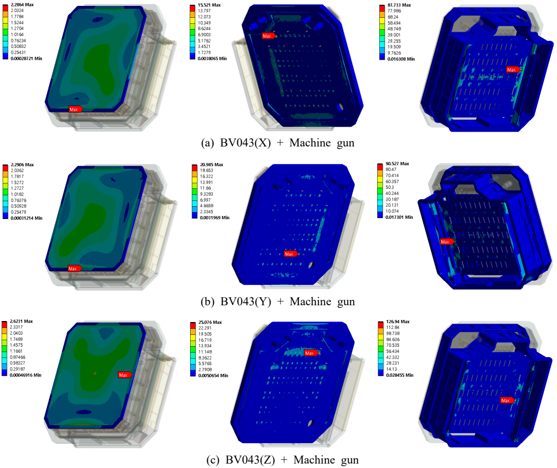
Fig. 8 Stress distribution for shock loads direction
